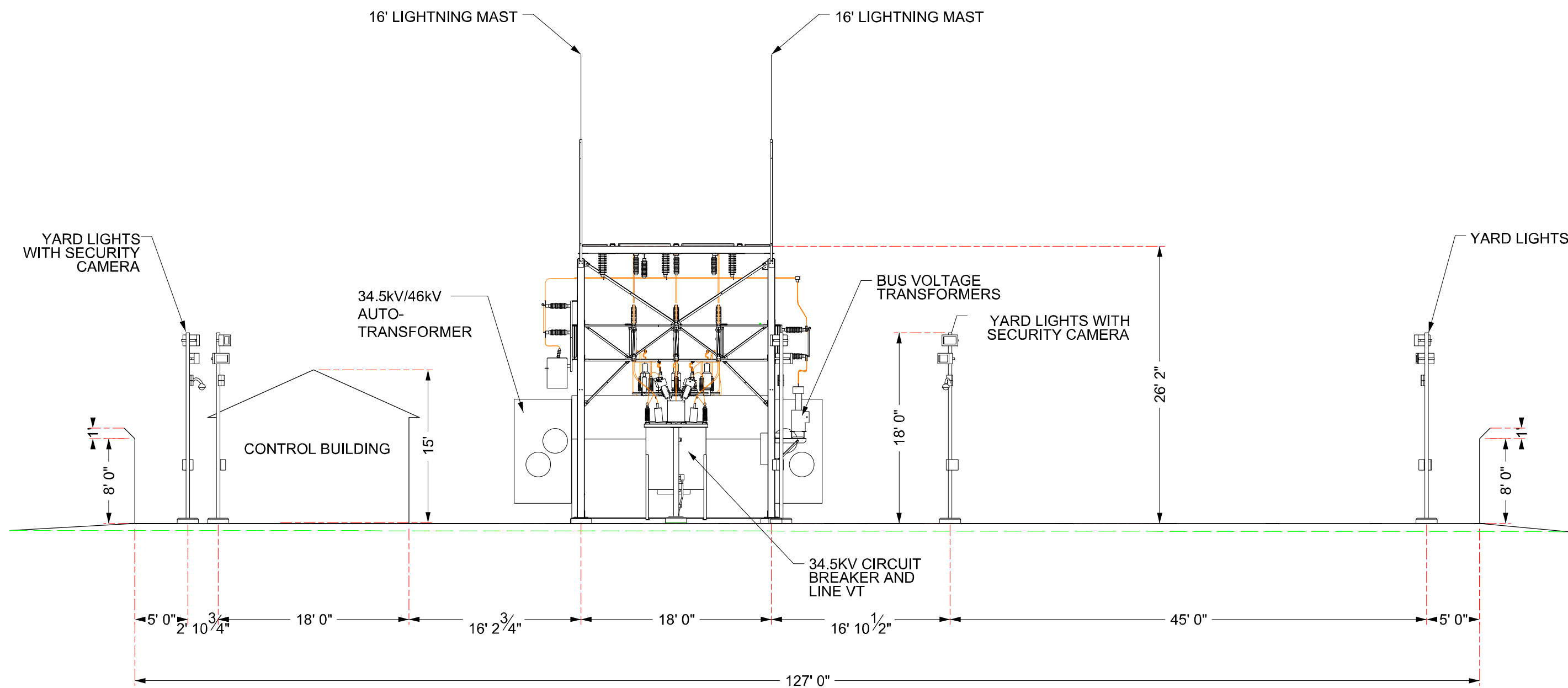
WEST ELEVATION - CC (FACING EAST)
