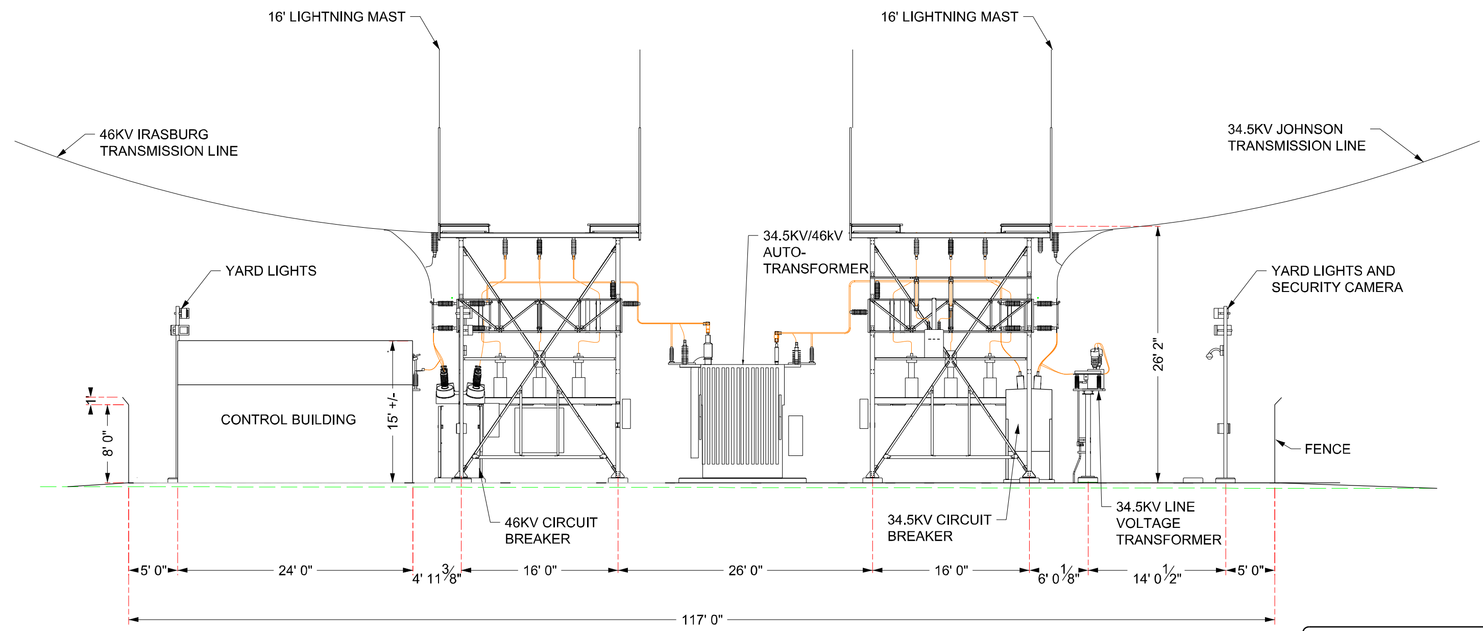
NORTH ELEVATION - DD (FACING SOUTH)
