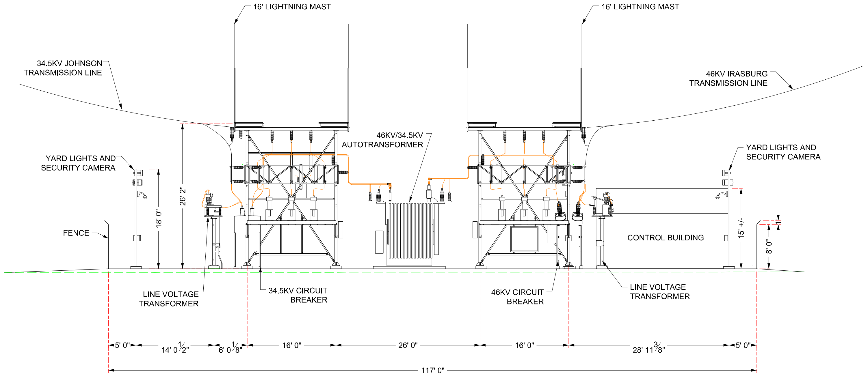
SOUTH ELEVATION - AA (FACING NORTH)
