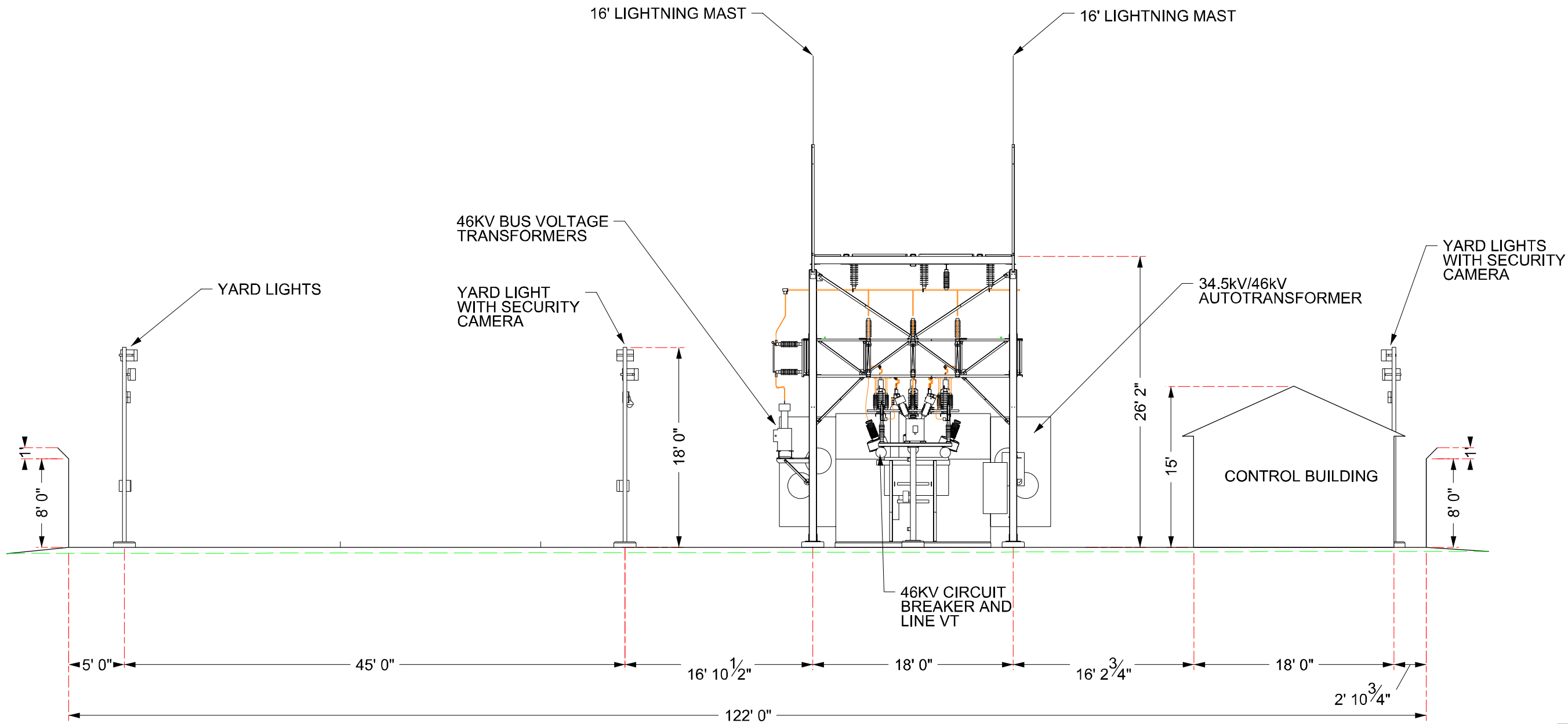
EAST ELEVATION - BB (FACING WEST)
